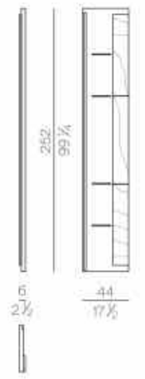
Lateral shoulder (left) NOVA.LS.SX.44
